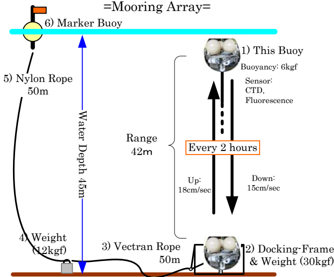
=Mooring Array=
